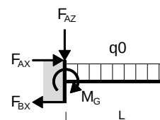
Belasting 3
