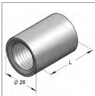
Overgooimoer
