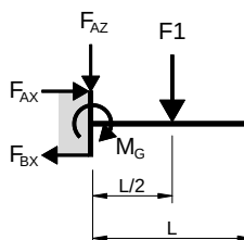
Belasting 1 (LF1)
