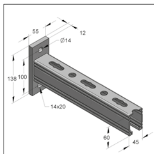
Console C-profiel 45/60/3,0 mm
