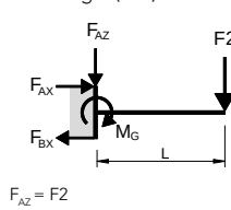
Belasting 2 (LF2)
