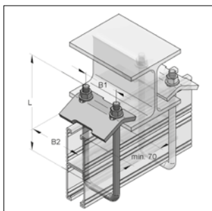
balkklemset M10 45/90
