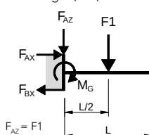
Belasting 1 (LF1)
