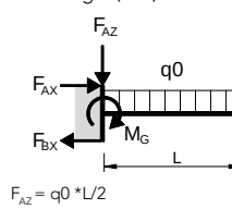
Belasting 3 (LF3)
