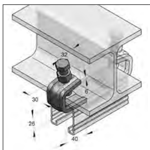
Rail balkklem
